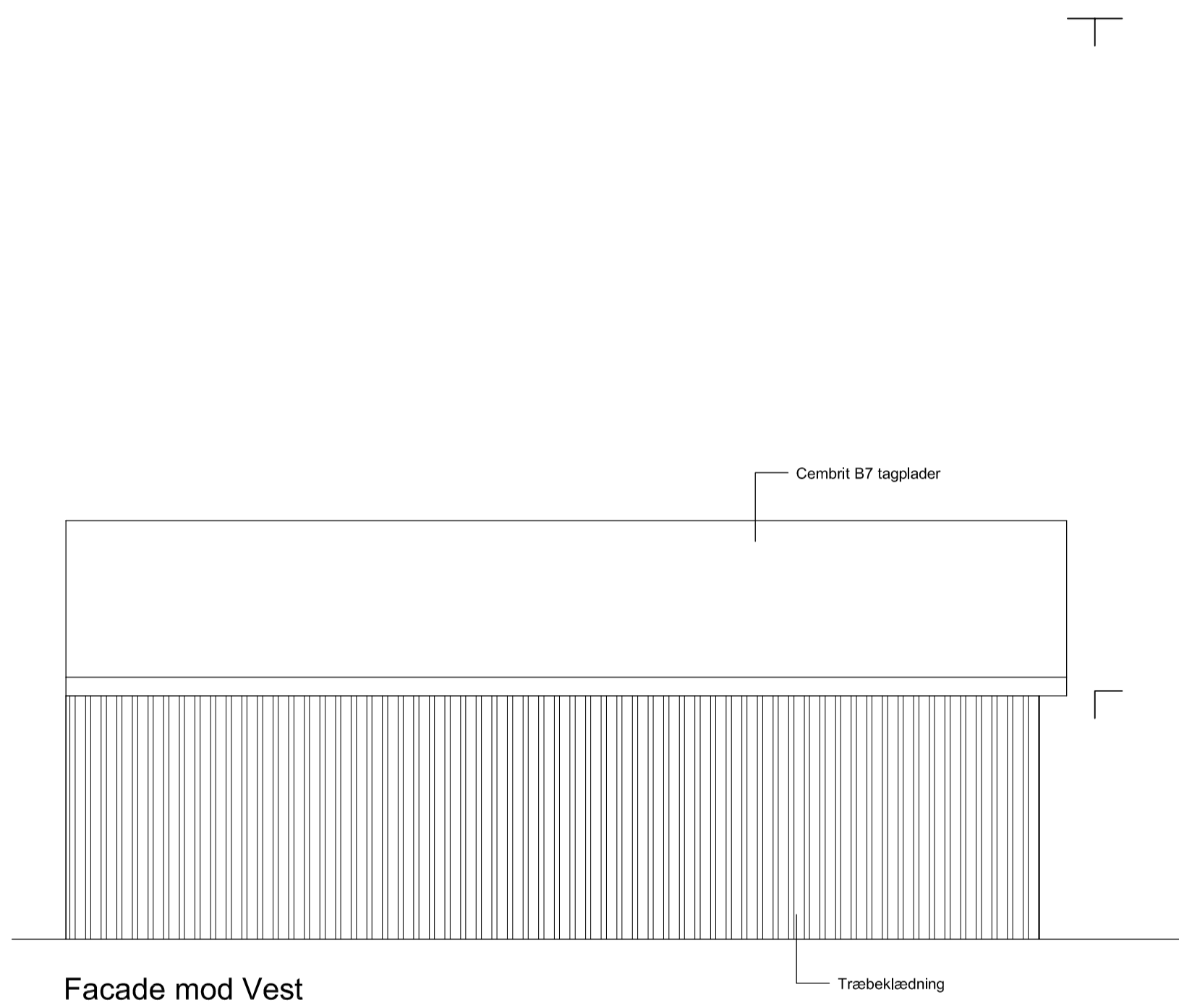
Facade mod Vest
